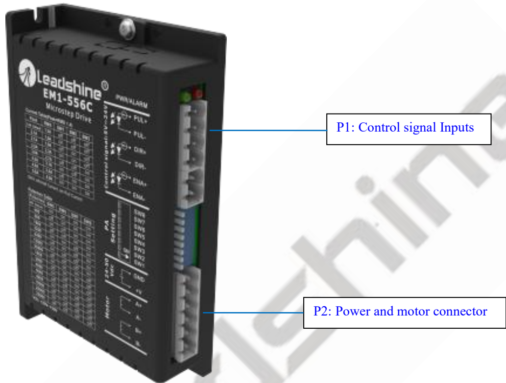
Figure 3 Connectors, DIP switches, and LED locations
