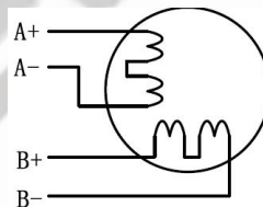
Figure 6 4-lead Motor Connections
