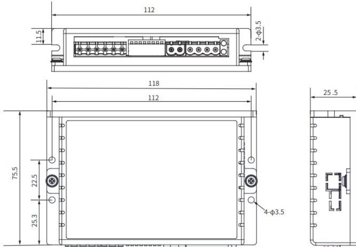
• Figure 1 EM1-442C, EM1-542C, EM1-556C Installation Dimension Drawing
