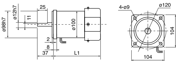
齿轮减速马达: GEARMOTOR
