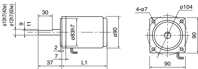
齿轮减速马达: GEARMOTOR
