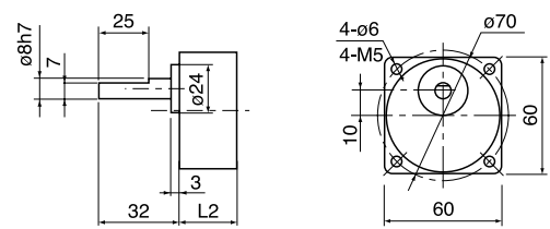
齿轮减速器: GEAR HEAD
