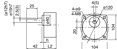
齿轮减速器: GEAR HEAD
