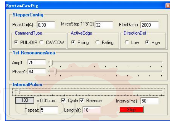
Figure 26: Anti-resonance tuning
