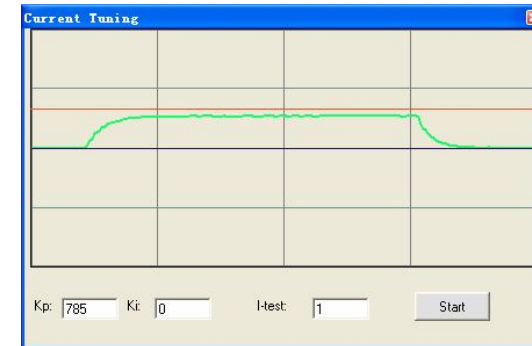
Figure 23: Kp=785, Ki=0 (poor performances)
