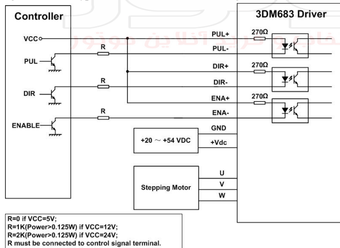
Figure 9: Typical connection
