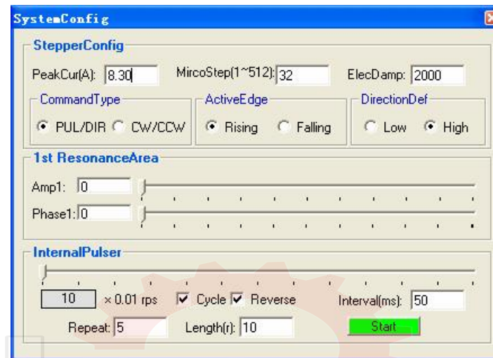
Figure 25: SystemConfig window
