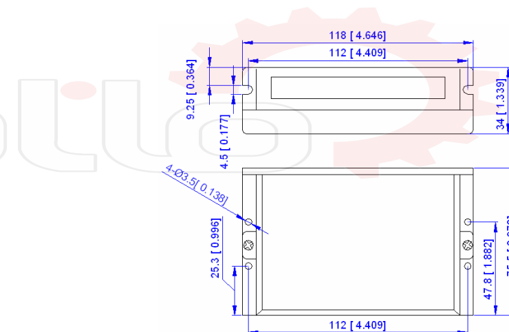
Figure 1: Mechanical specifications
