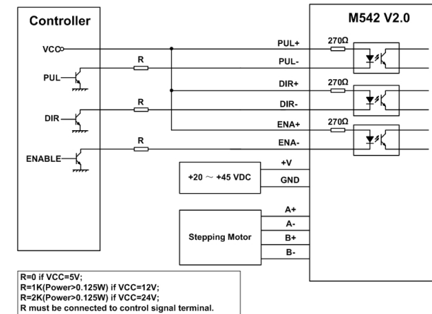
Figure 10: Typical connection
