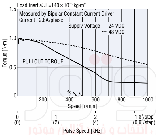
● PK268DAT Bipolar
