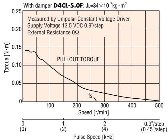
● PK243M-03B Unipolar
